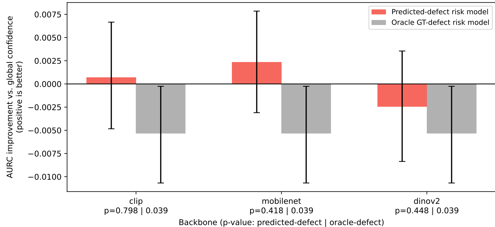
Selective Prediction Diagnostic: Defects Do Not Improve Risk Ranking
